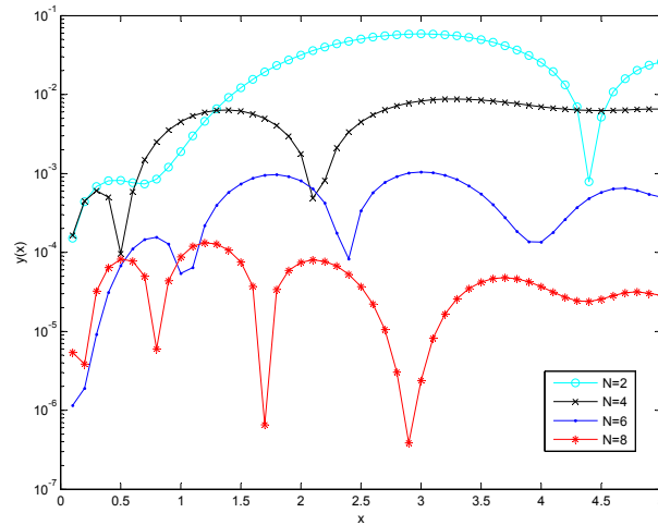
FIGURE 1. Error between the exact- and numerical solutions of our method for g(x) = x^2 and various of N , in Example 5.1.
