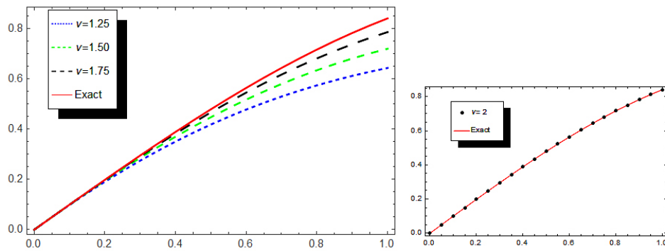
FIGURE 9. Comparison of y(x) for m = 3 , with \nu = 1.25, 1.50, 1.75, 2 and the exact solution for Example 6.6.
