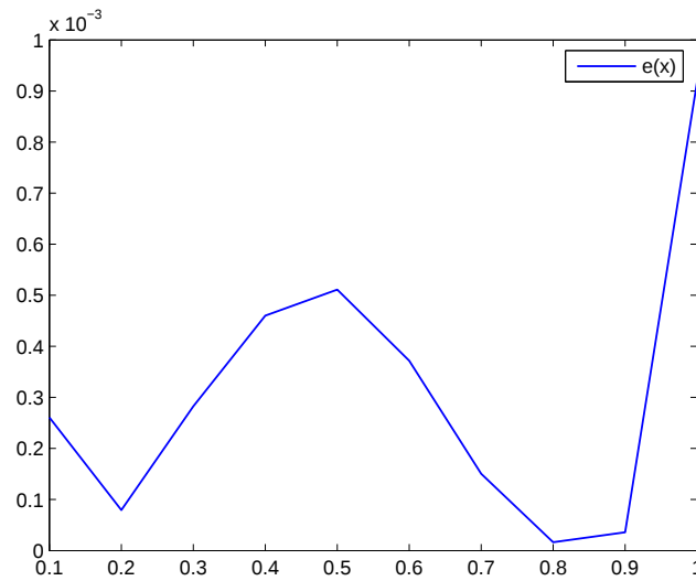
FIGURE 6. The error function of Example 4.
