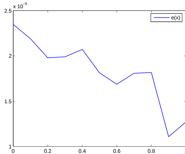
FIGURE 5. The error function of Example 3.
